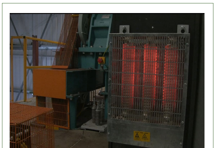
Before: Excess Energy Lost Through Braking Resistors
